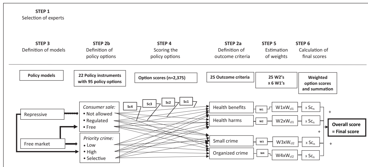
Figure 1. The six steps of the multi-decision multi-criterion decision analysis. W_{c1} to W_{c6} represent the six cluster weight factors; W1 \times W_{c1} (in Table 3 described as W1 \times W2 ): 25 overall weight factors; Sc_n to Sc_{n+1} are the scores for the policy options obtained in step 4; multiplication of the overall weight factor of the criterion with Sc_n gives the weighted option score. Summation of 22 weighted selected policy options gives the overall score (final score) of a constructed model.
