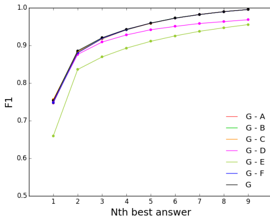
Figure 2: Ablation study on feature sets.
