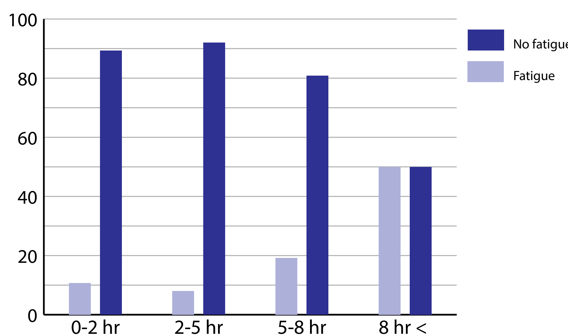
Figure 1: Distribution of fatigue as contributory factor with respect to flight duty times.
