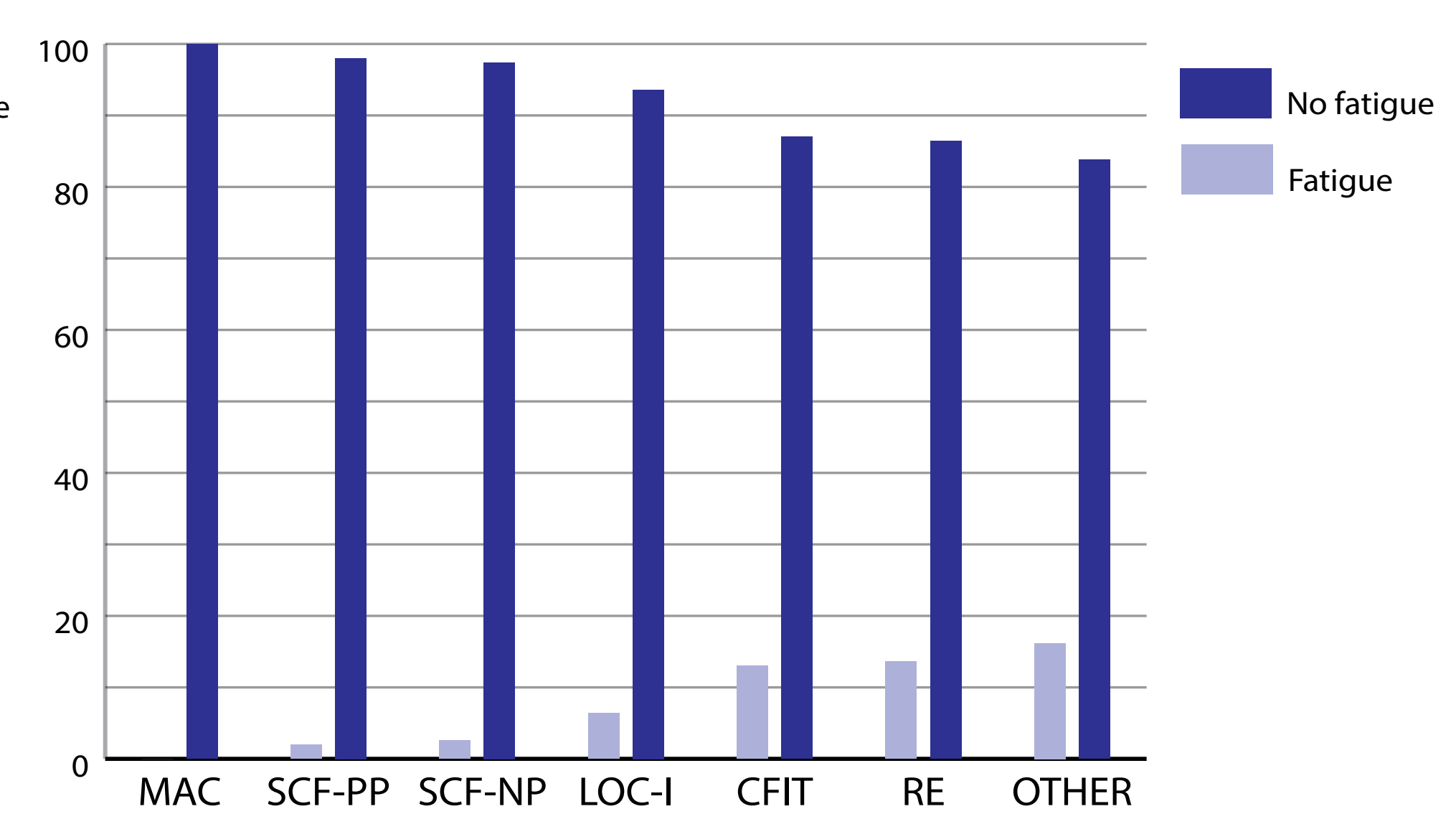
Figure 2: Distribution of fatigue as contributory factor in various event categories. Note: CFIT (Controlled Flight into Terrain), LOC-I (Loss of Control - in-flight), MAC (Mid-air Collision), RE (Runway Excursion), SCF-NP (System/component failure - Nonpowerplant), SCF-PP (System/component failure - Powerplant)
