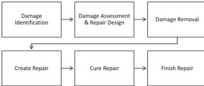
Figure 7: Typical MRO composite repair process (Borst et al., 2020)
