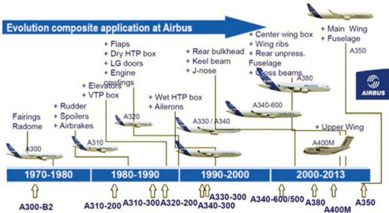
Figure 5: Evolution in composites aircraft applications (Airbus, 2013)
